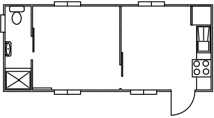
6x3m Accommodation Unit
