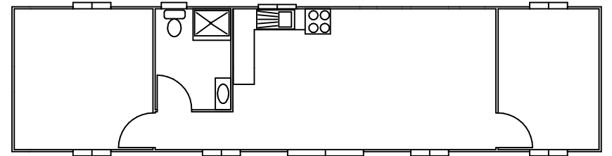
14x3.4m Accommodation Unit
