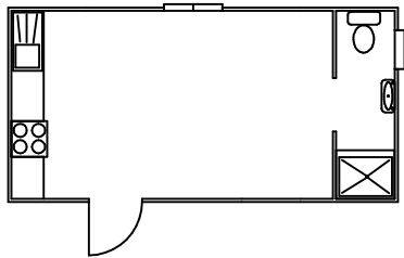
6x3m Accommodation Unit
