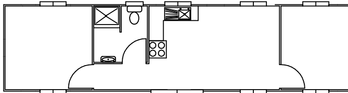
12x3m Accommodation Unit
