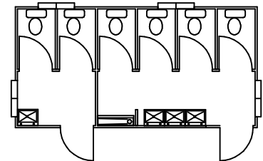
6x3m M/F Ablution
